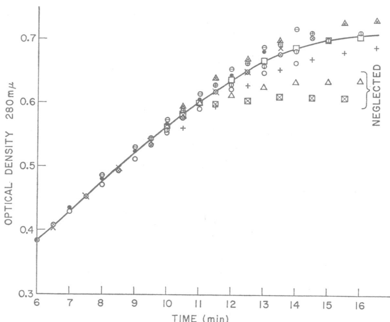
FIGURE 16 Tase reaction rates at 25°C. Effect of magnetic field of 170,000 gauss. Simulated runs, 3 min exposure: ○ and ⊗, magnet and control; ● and ×, magnet and control. Magnet runs, 3 min exposure: ⊕ and +, magnet and control; ⊖ and ⊕, magnet and control. Simulated run, 7 min exposure: △ and ▴, magnet and control. Magnet run, 7 min exposure: □ and ▣, magnet and control. Enzyme concentration 9.7 \times 10^{-2} mg/ml before adding substrate. Reactions placed in magnet at 2 min.
