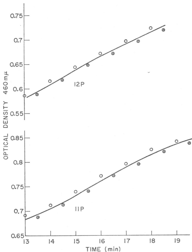
FIGURE 15 Pase reaction rate at 25°C. Effect of magnetic field. \circ , magnet; \otimes , control. 12P, 10 min exposure to 85,000 gauss; 11P, 10 min exposure to large field gradient. Enzyme concentration 7.5 \times 10^{-6} mg/ml in reaction mixture. Reactions placed in magnet at 2 min.
